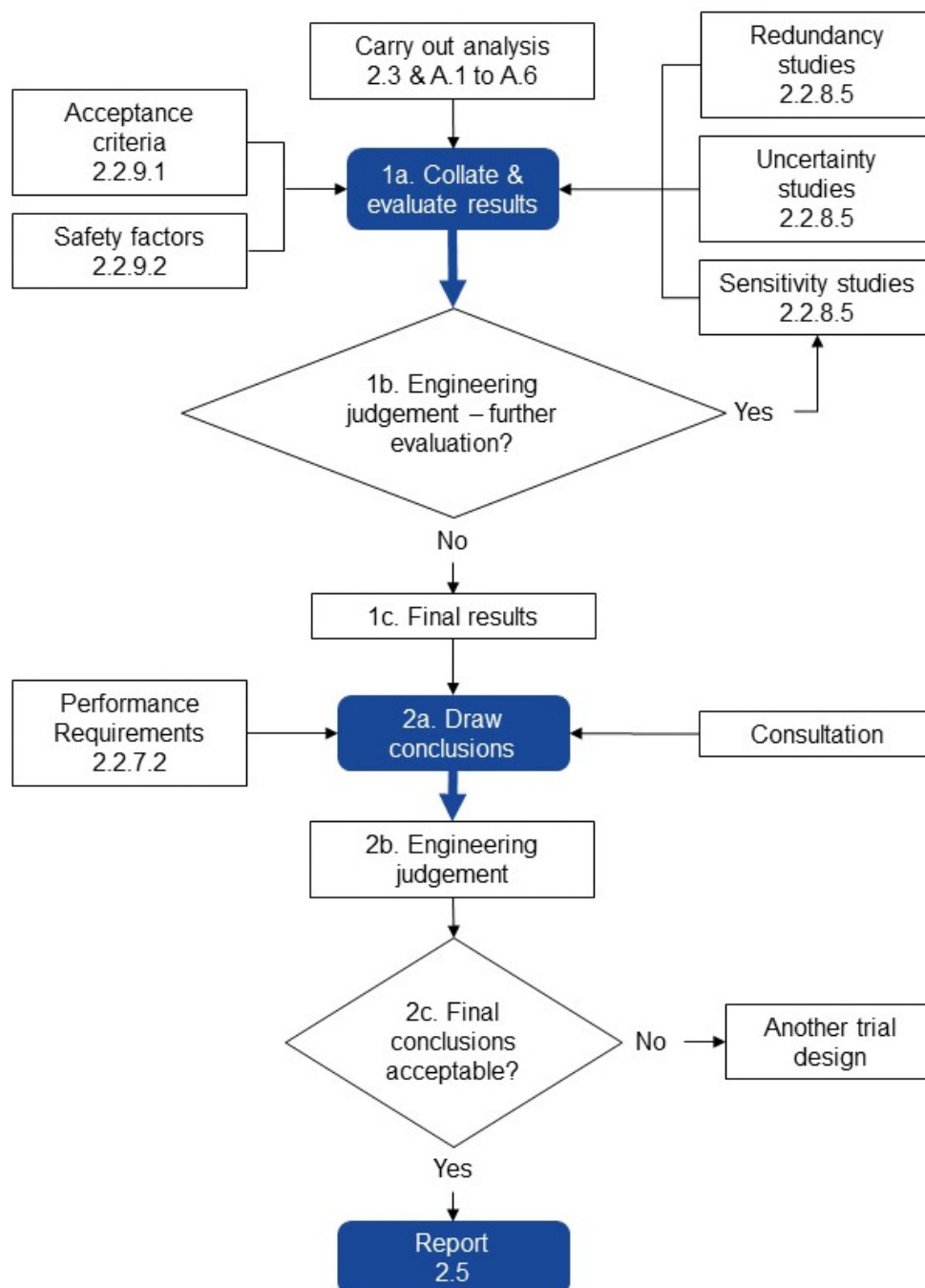
Figure 2.4.1 Flow chart for collating and evaluating the results and drawing conclusions
