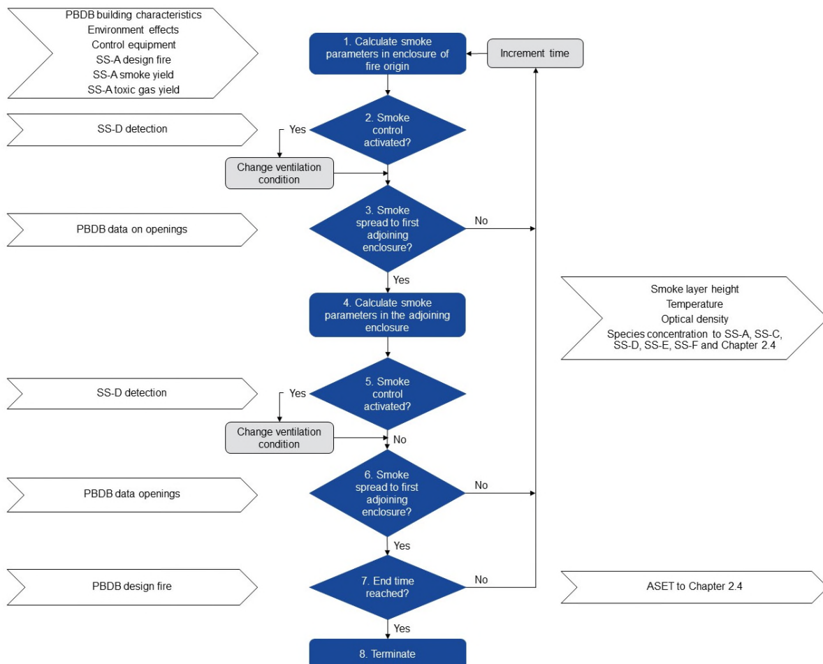
Figure A.2.1 Flow chart for smoke development and spread analysis
