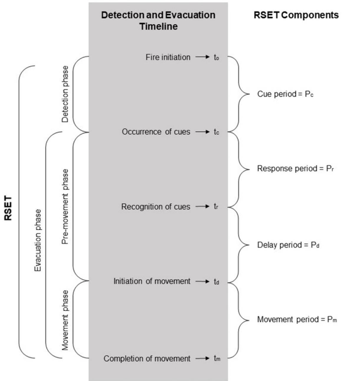
Figure A.5.1 Detection and evacuation timeline
