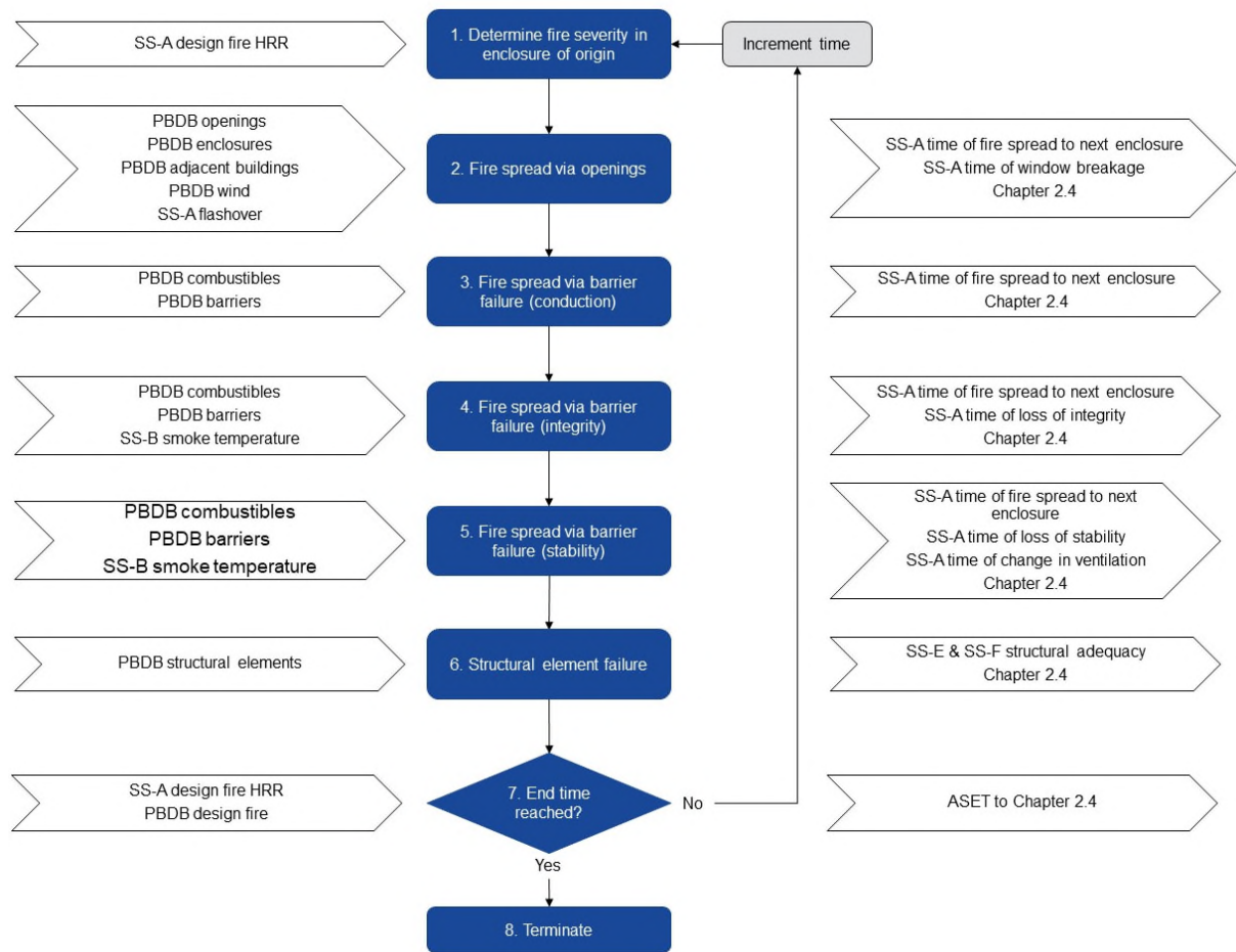
Figure A.3.1 Flow chart for fire spread and impact analysis
