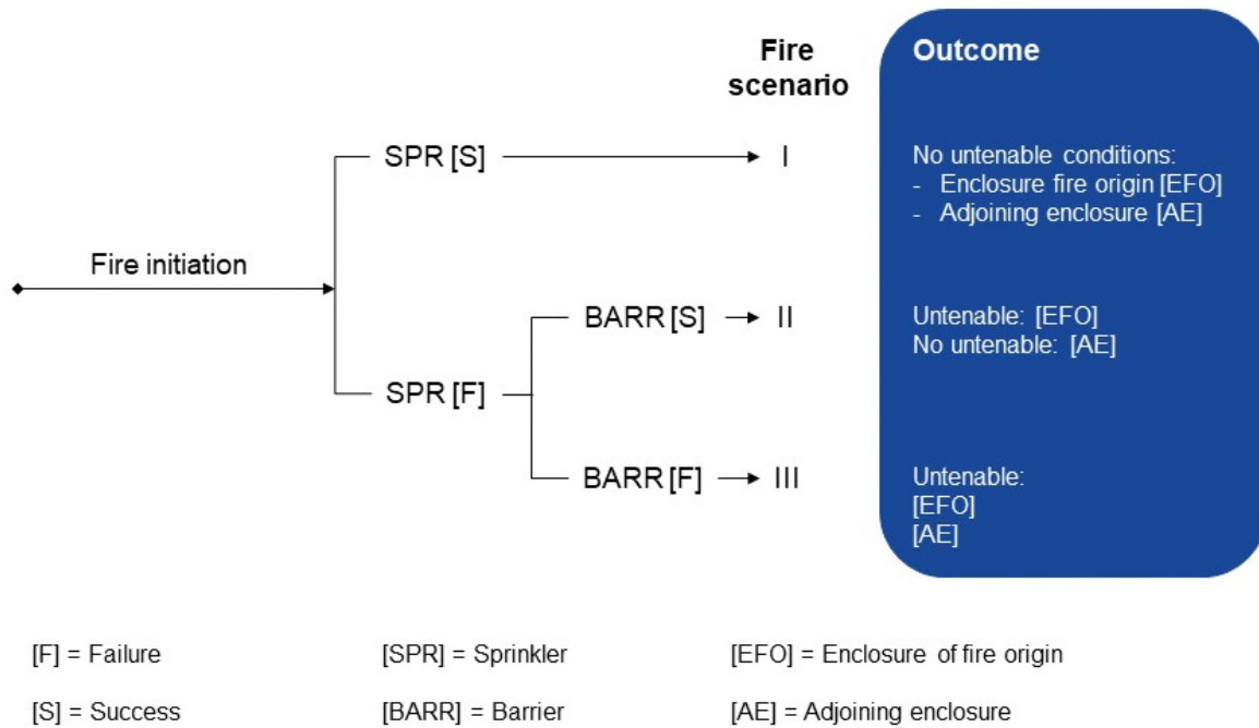
Figure 3.1.1 Event tree representation of the possible events associated with a fire safety system including sprinklers and barriers
