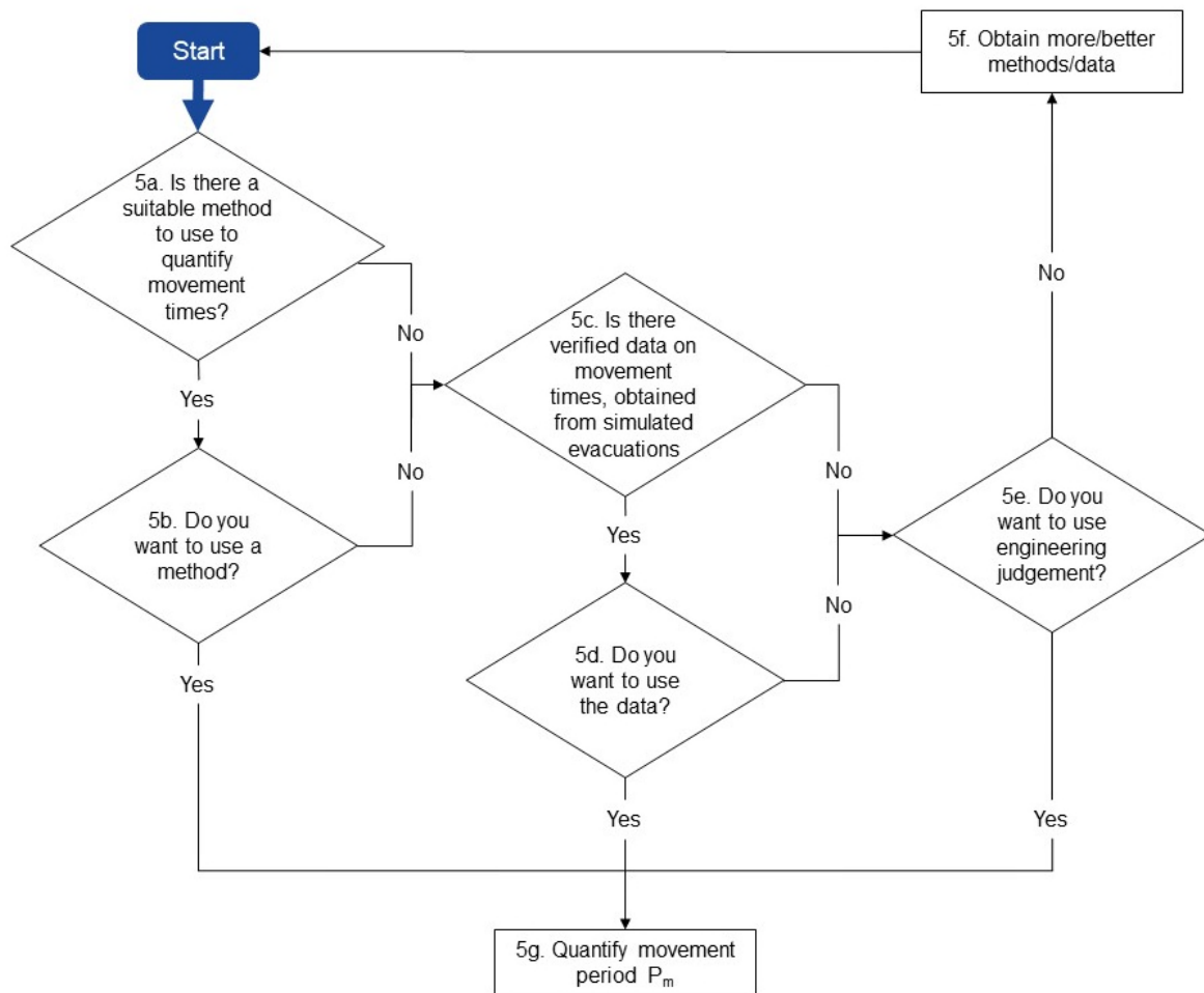
Figure A.5.6 Flow chart for determining the movement period ( P_m )
