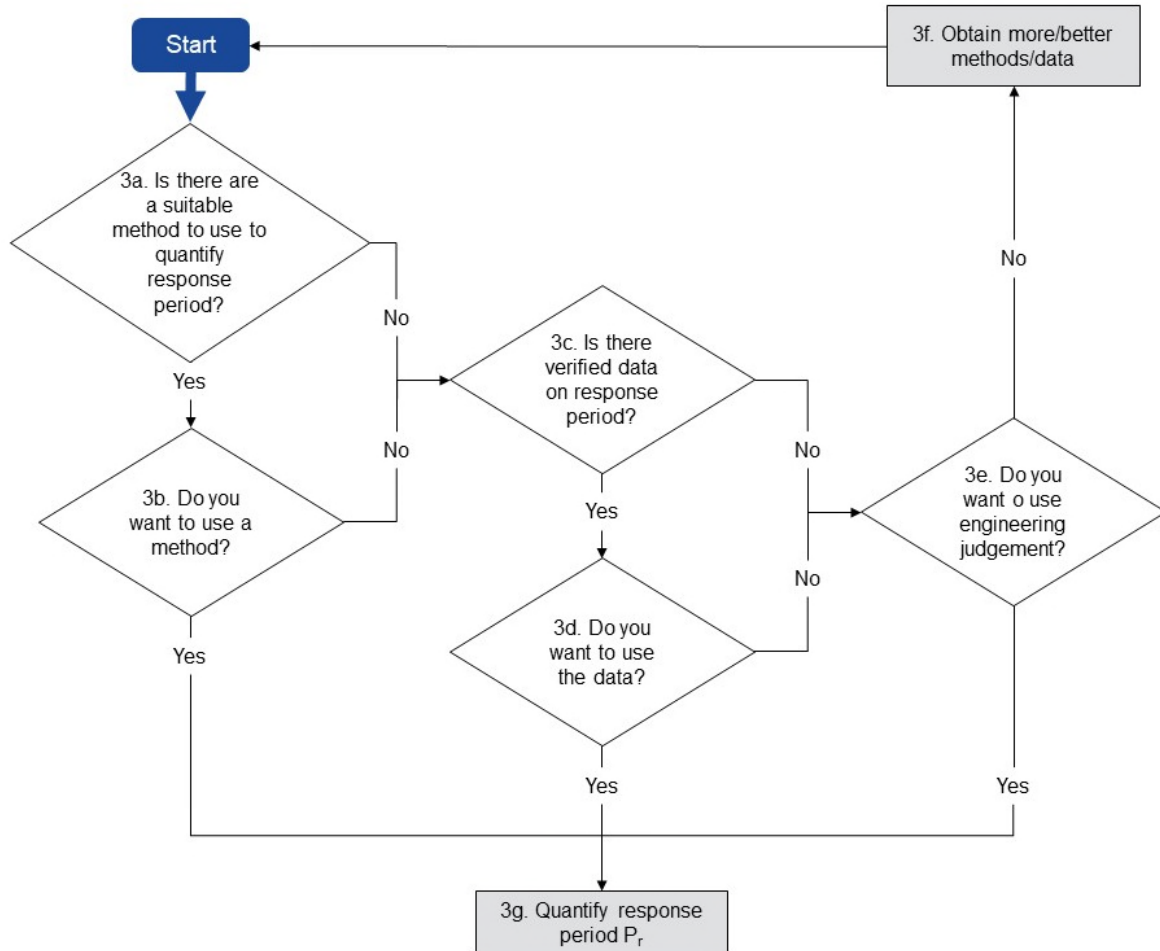
Figure A.5.4 Flow chart for determining response period ( P_r )
