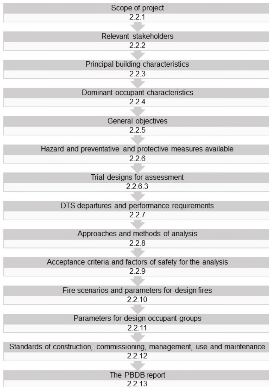
Figure 2.2.1 A process for developing a PBDB
