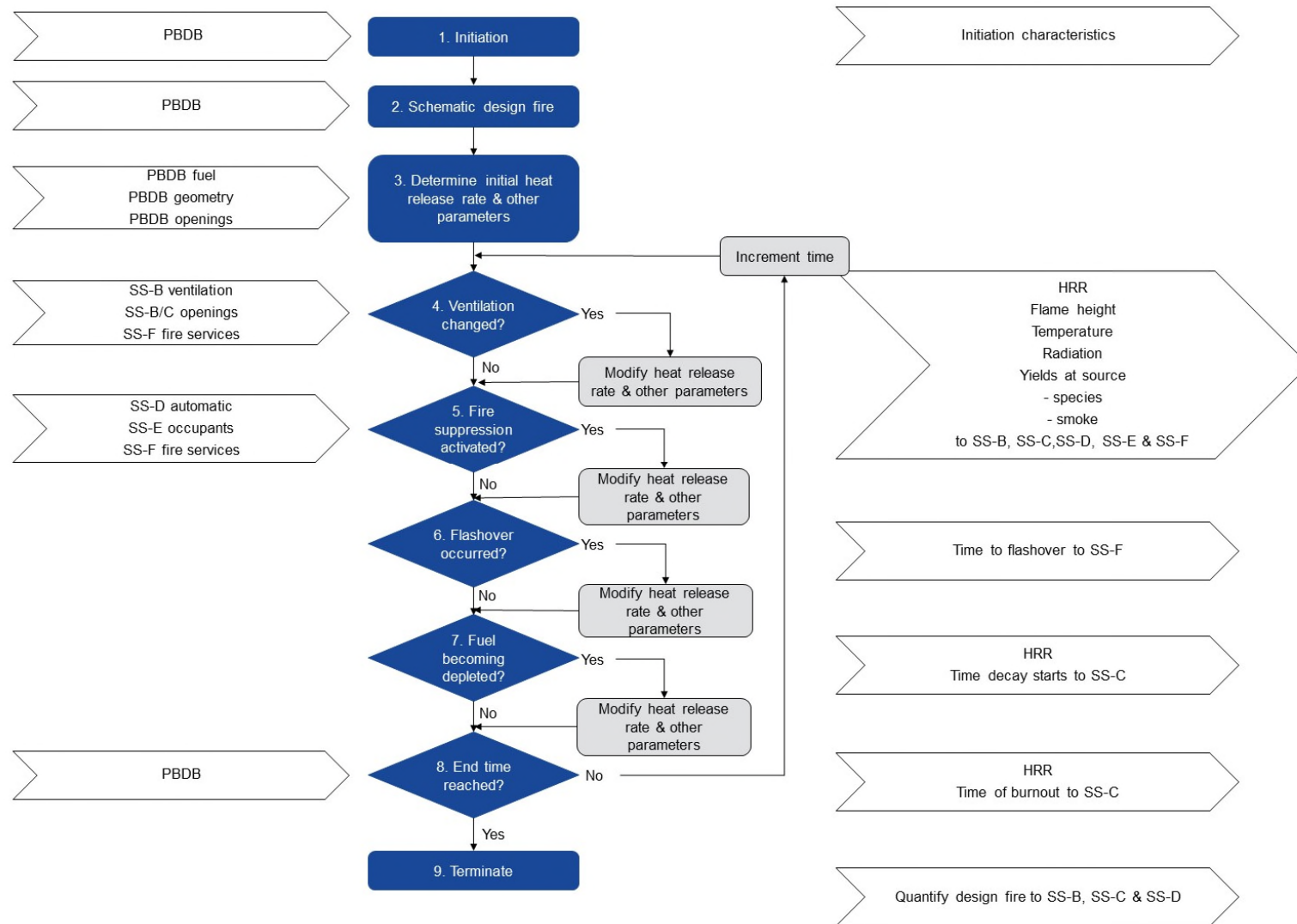
Figure A.1.1 Flow chart for fire initiation and development analysis
