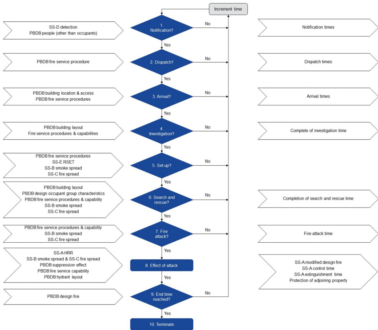
Figure A.6.1 Flow chart for fire services intervention analysis
