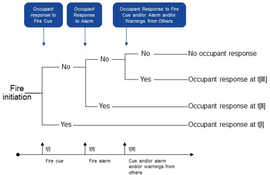
Figure 3.1.3 Occupant responses based on an event tree formulation plus associated timeline
