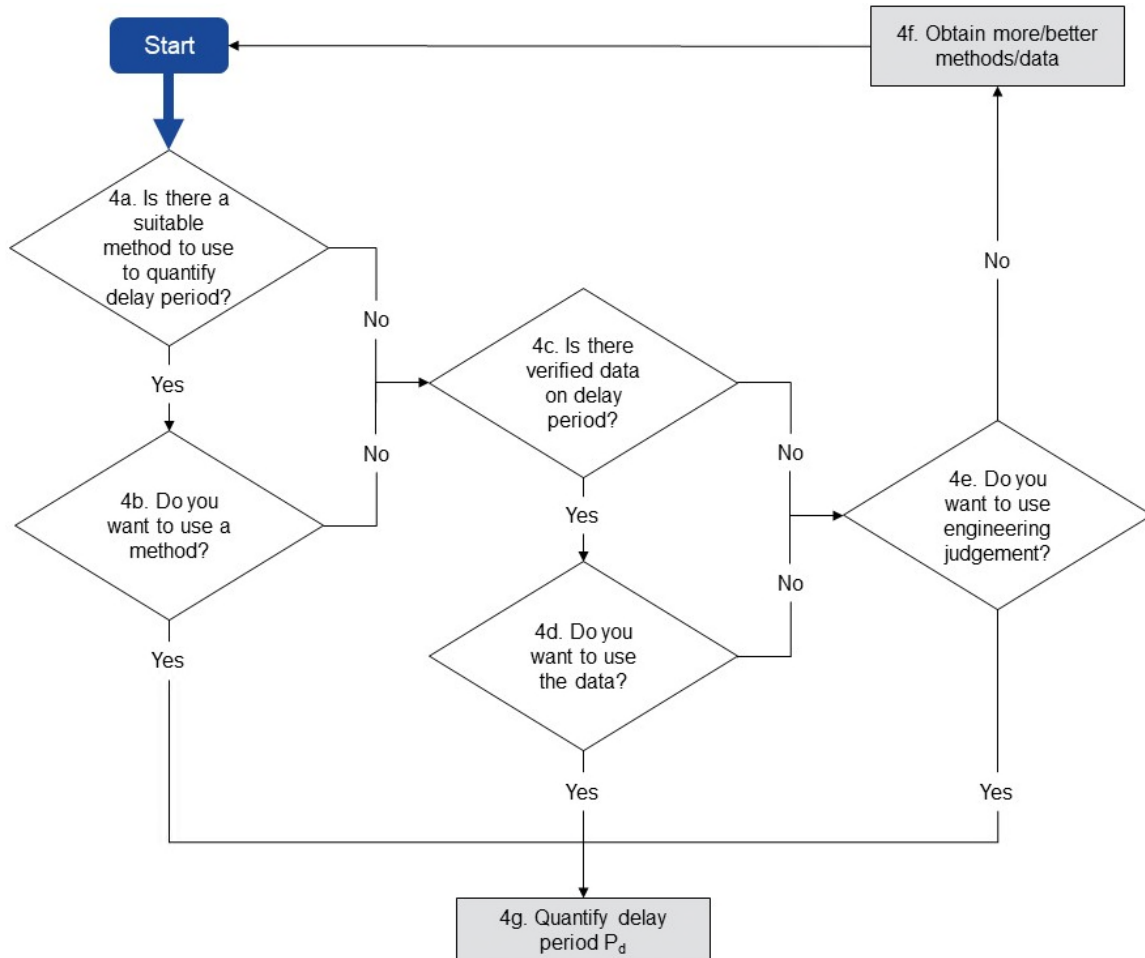
Figure A.5.5 Flow chart for determining the delay period ( P_d )
