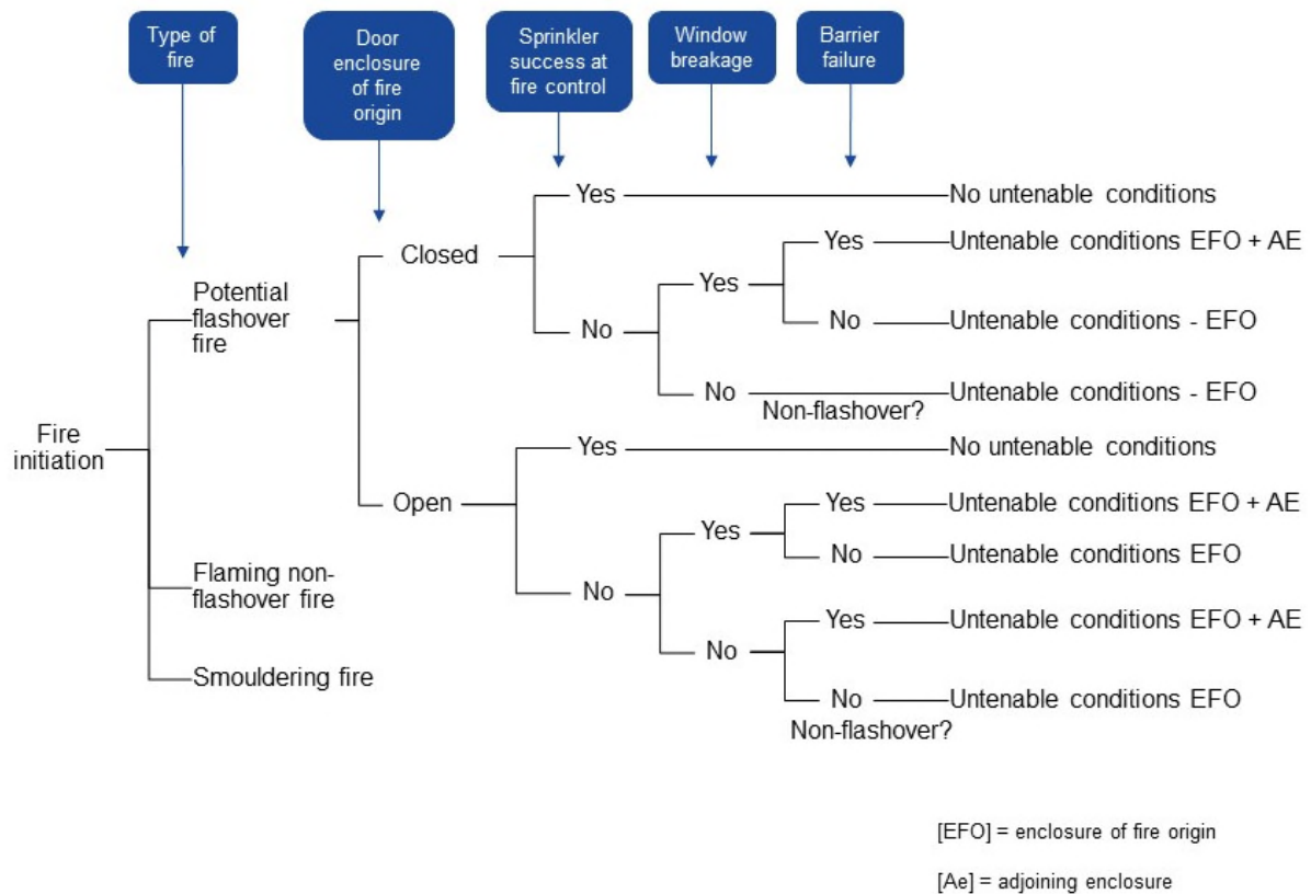
Figure 3.1.2 Fire scenarios using an event tree approach
