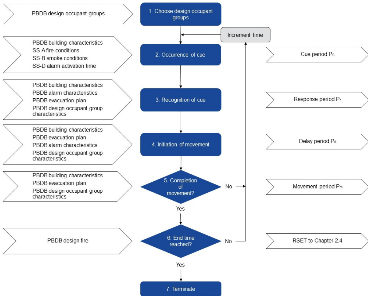
Figure A.5.2 Flow chart for occupant evacuation analysis
