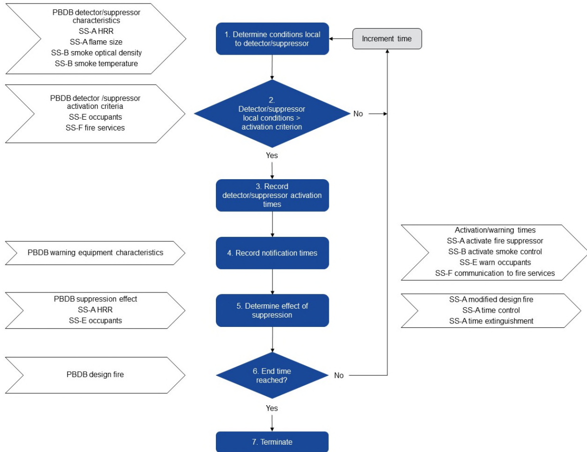
Figure A.4.1 Flow chart for detection, warning and suppression analysis
