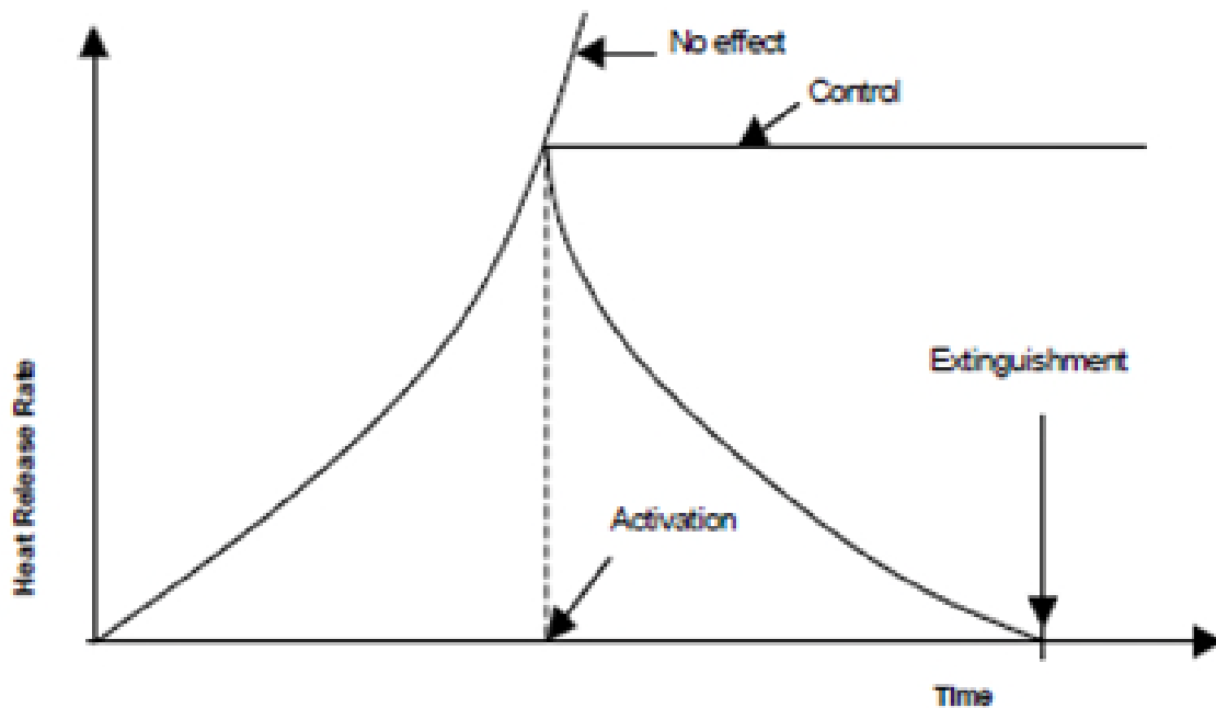
Figure A.6.2 Possible effects of suppression on a design fire
